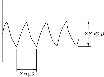
❶ IC801 ②⑩ (OSC IN)
