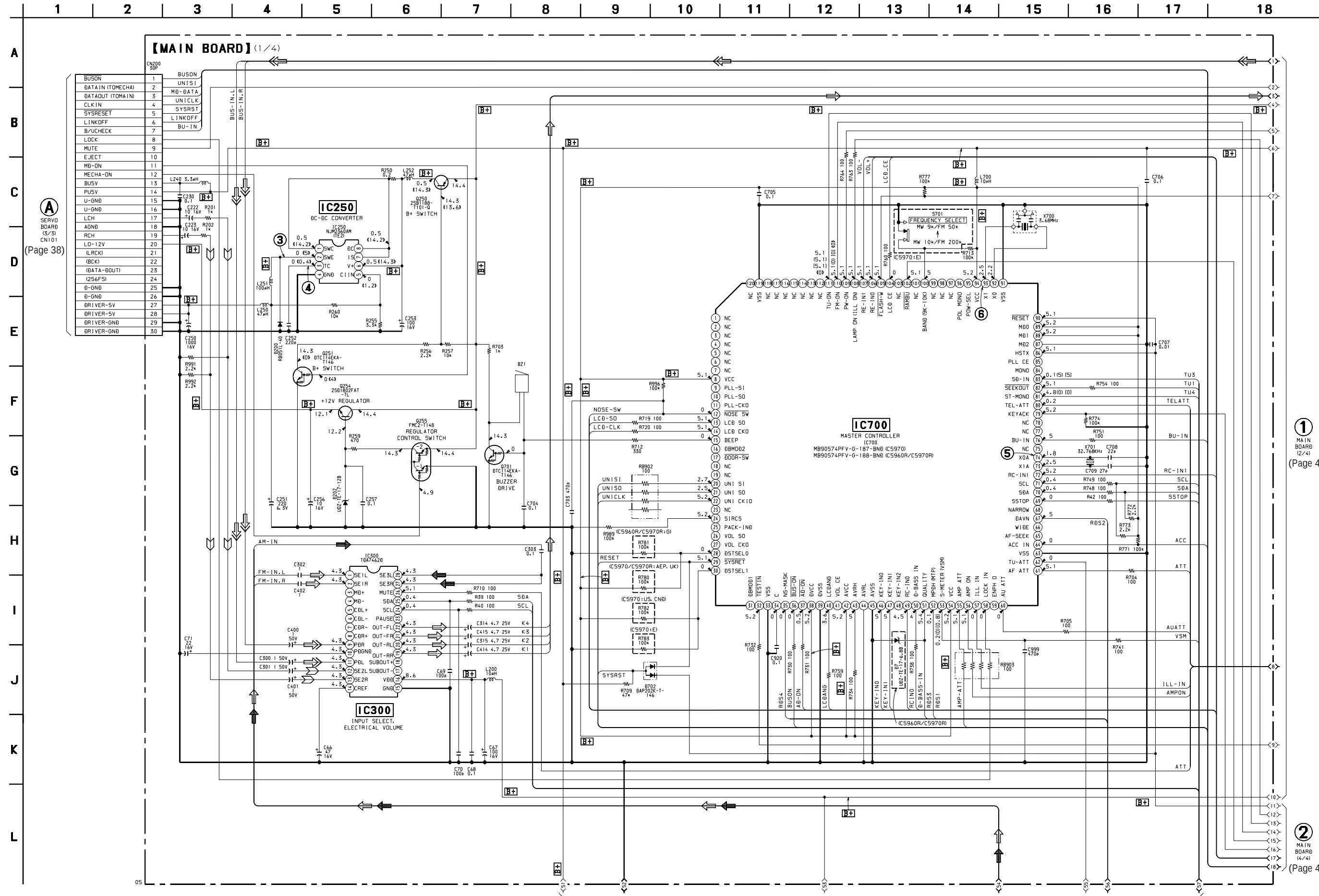
4-13. SCHEMATIC DIAGRAM – MAIN Board (1/4) – • See page 55 for Waveforms. • See page 60 for IC Block Diagrams.
