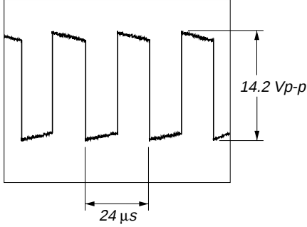
❹ IC250 ③ TC (MD PLAY Mode)
