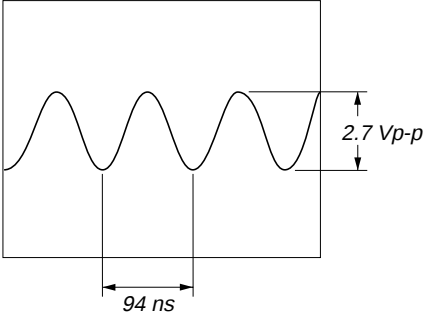
❷ IC102 ⑤ (OSC1) (FM Mode)
