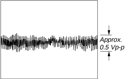
❶ IC302 ②⑥ (TE) (MD PLAY Mode)
