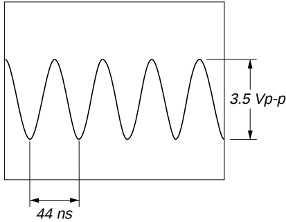
❼ IC304 ③ (IN) (MD PLAY Mode)
