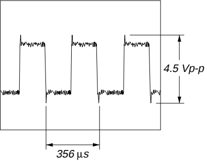
❺ IC301 ②⑥ (XBCK) (MD PLAY Mode)
